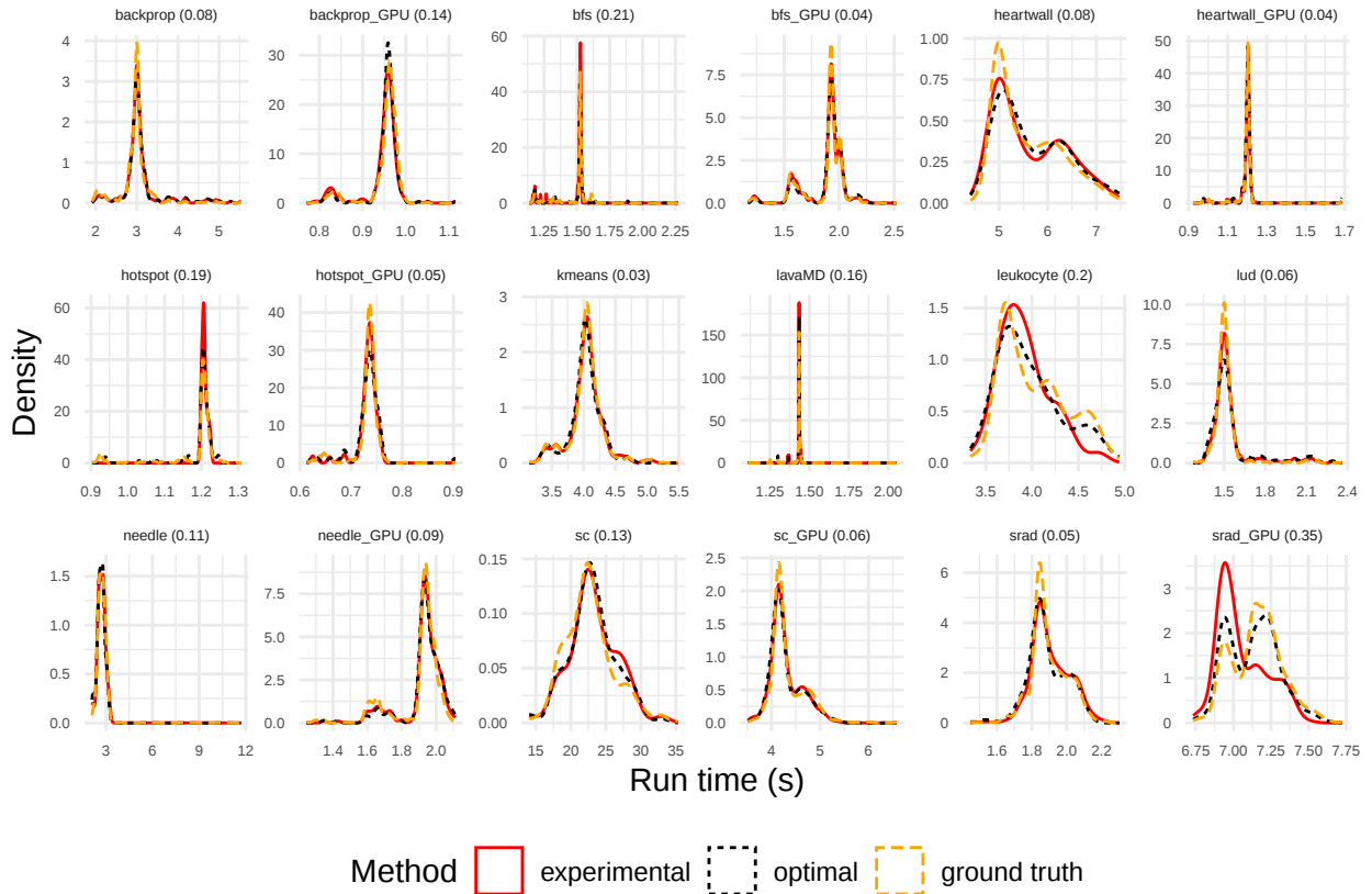
Figure 5: Density plots of Rodinia benchmark distributions using three methods of generation. Each distribution name is followed by KS distance of the experimental sample relative to the ground truth.
