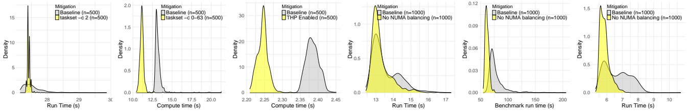
(a) 7z (thread pinning) (b) lbm (thread pinning) (c) sad (transparent huge pages) (d) Xapian (disabling NUMA balancing) (e) srad (disabling NUMA balancing) (f) lavaMD (disabling NUMA balancing)
