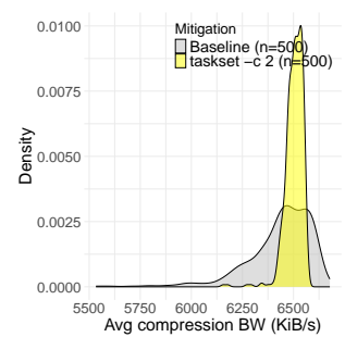
Figure 11: Impact of pinning on 7z
