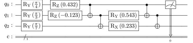
Fig. 1. Parametrized Quantum Circuit (PQC) used in the experiments.
