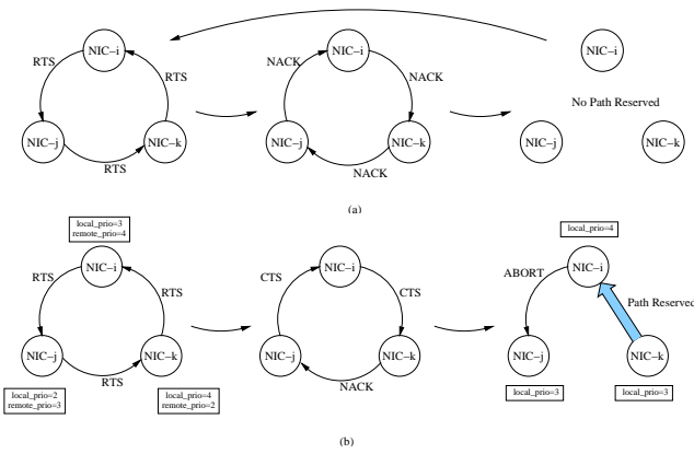
Figure 2. Deadlock example
